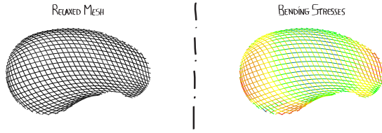
Fig. 10. Geometry of the relaxed mesh and its bending stresses diagram. The calculations, performed numerically thanks to a dynamic relaxation algorithm with kinetic damping [14], is composed of the following steps:
